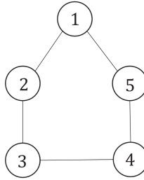
Fig. 1. The communication graph for the players.
