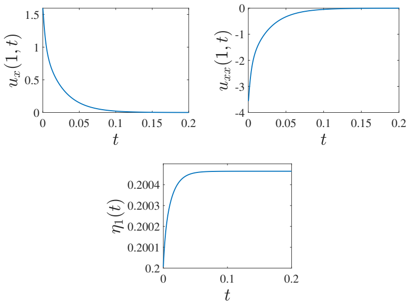
Fig. 7. Boundary controls (100), (101) and update law (102).
